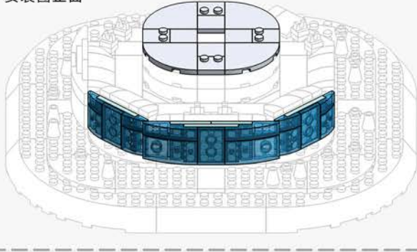
Front Side of Installation Drawing 安装图正面
